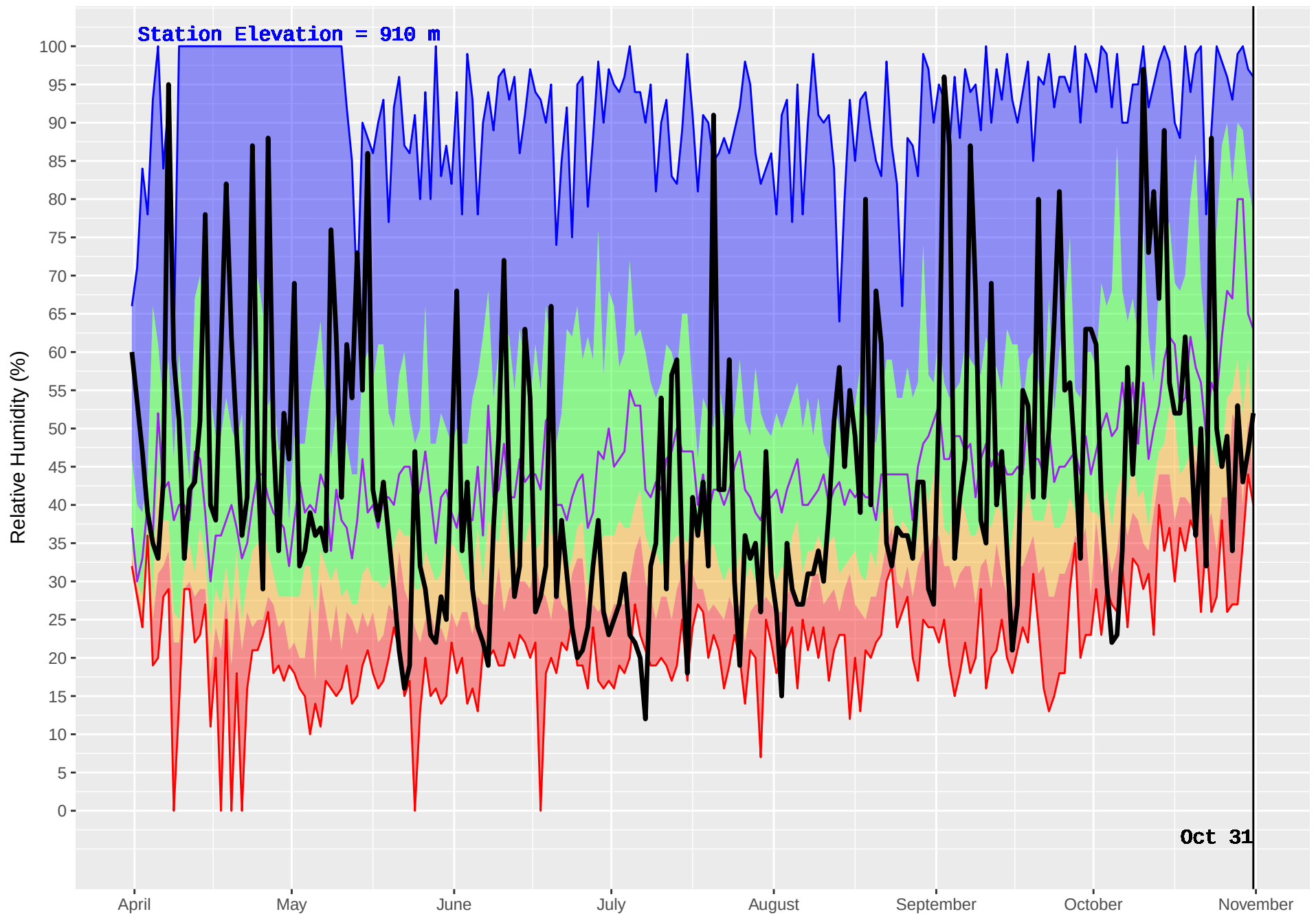
NAZKO (211) : Historical (1981–2016) and Current (2017) Noon Relative Humidity
