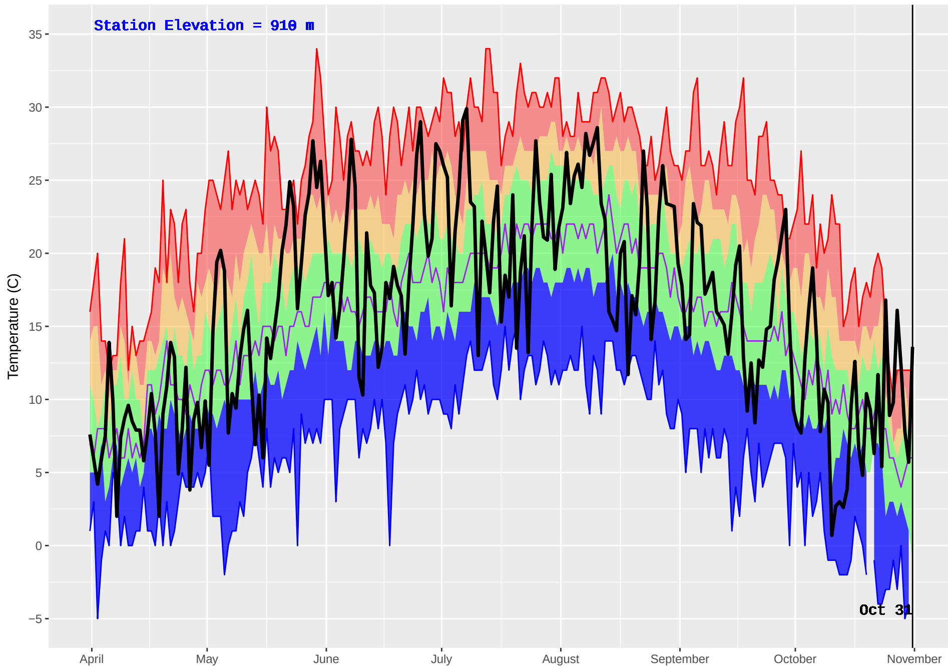
NAZKO (211) : Historical (1981–2016) and Current (2017) Noon Temperature
