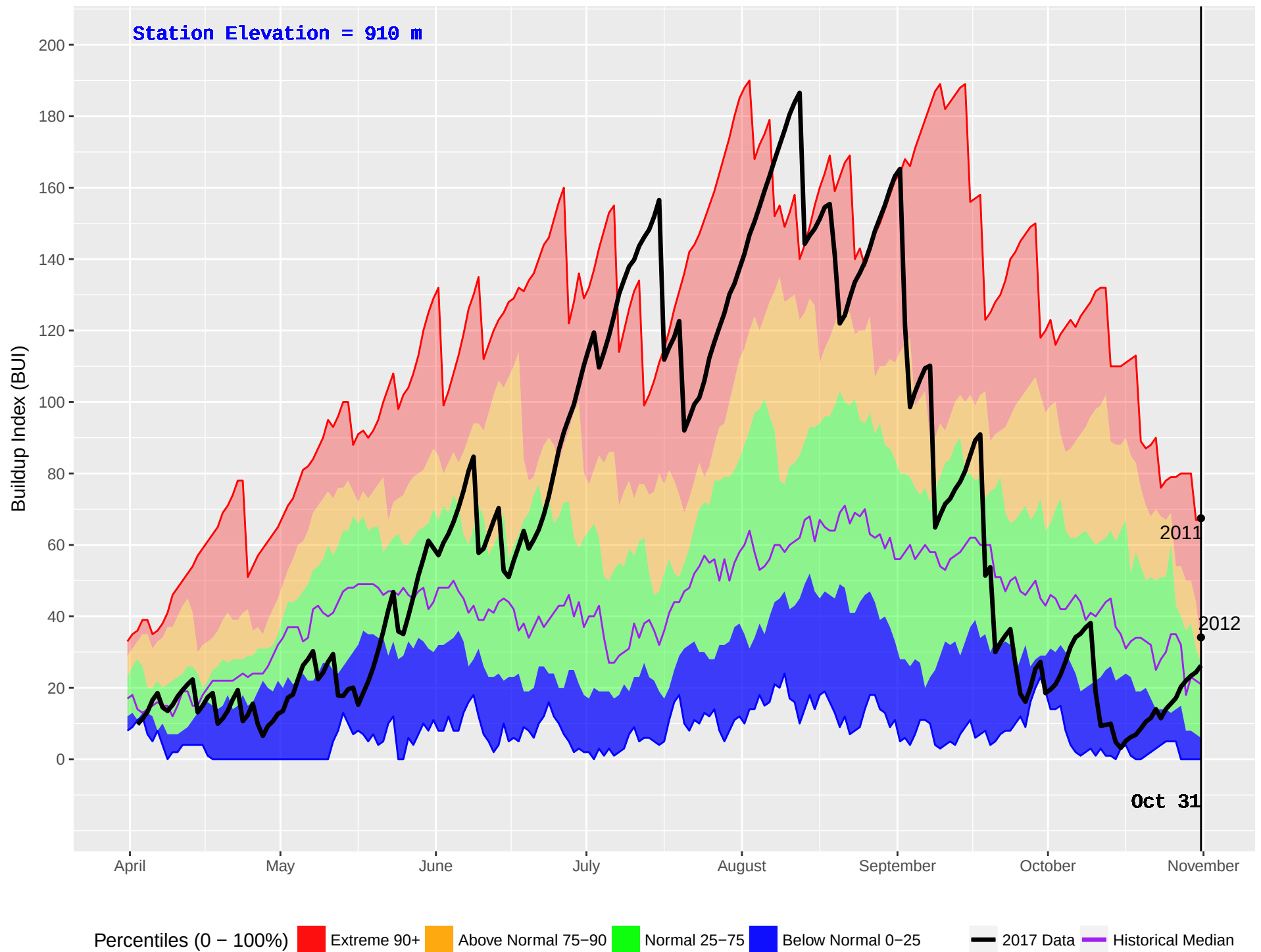
NAZKO (211) : Historical (1981–2016) and Current (2017) Noon Buildup Index (BUI)
