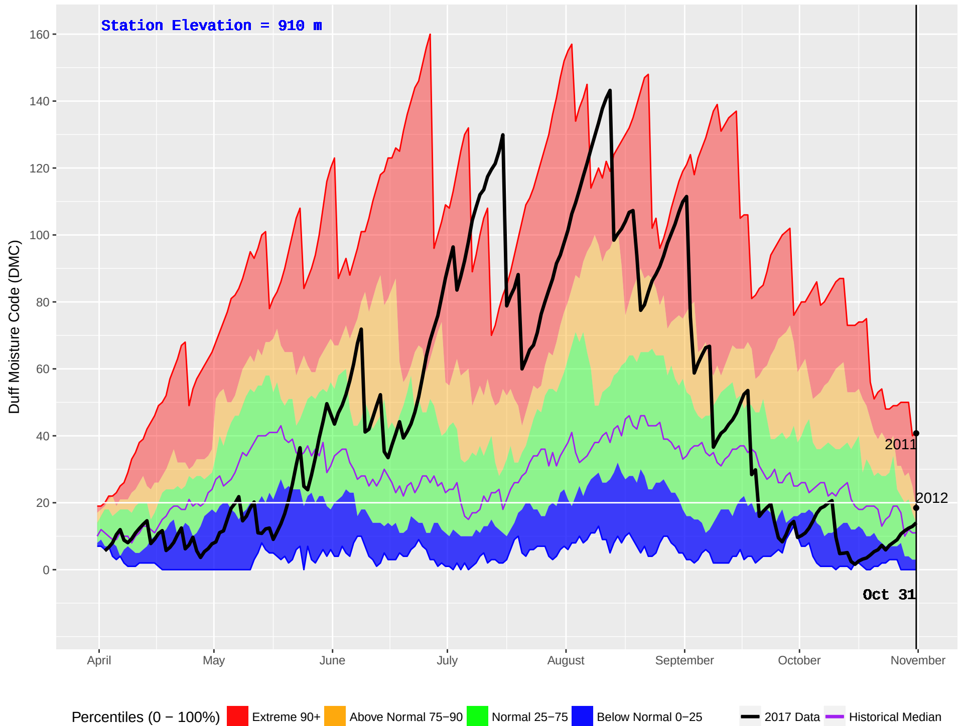
NAZKO (211) : Historical (1981–2016) and Current (2017) Noon Duff Moisture Code (DMC)
